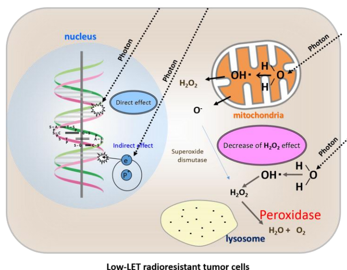
Figure 3. Direct effects, indirect effects, and a shortage of the “ \text{H}_2\text{O}_2 effect” of radiation therapy in low-LET radioresistant tumor cells.
