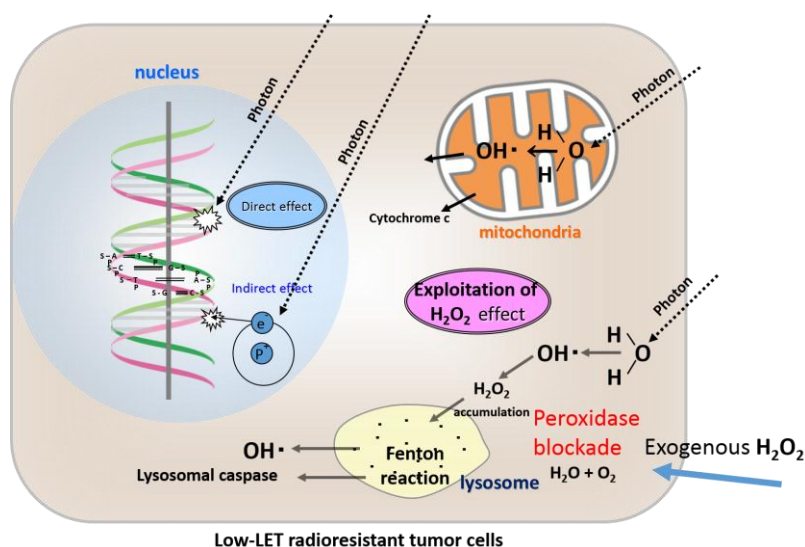
Figure 4. Direct effects, indirect effects, and an exploitation of our newly proposed “ H_2O_2 effect” by an exogenous H_2O_2 supply for low-LET radiation in chondrocytes and osteosarcoma cells in terms of blockade of high peroxidase activity and hyperoxia.
